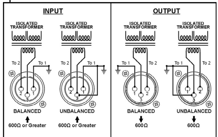
fig.3 XLR WIRING
